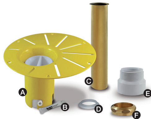
Drop-in drain (A), Lubricant (B), Brass tailpiece (C), Gasket (D), Adaptors 1 1/2" female (E) and Nuts (F)
